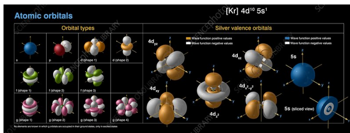
Atomic structure of Silver diagram
